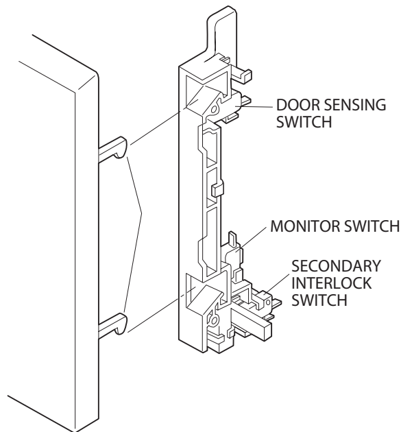
Figure C-4. Latch Switch Adjustments
