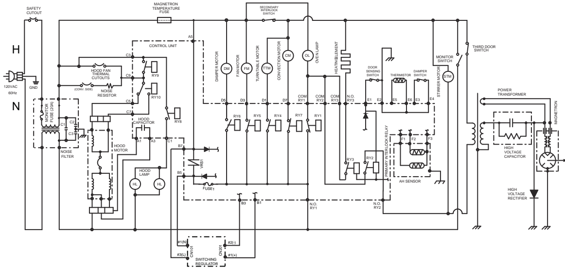
Figure O-3. Oven Schematic - Convection Cooking Condition (CONVEC, PREHEAT, BROIL, SLOW COOK)
