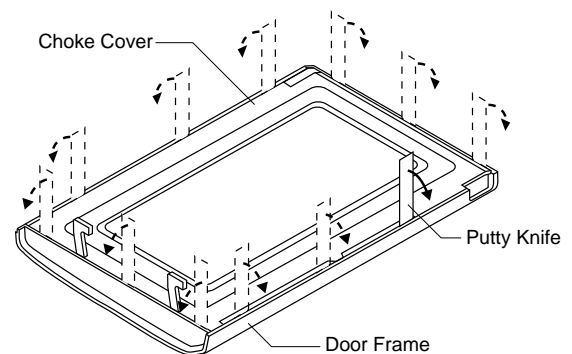
Figure C-6. Door Disassembly
