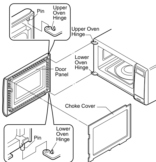
Figure C-7. Door Replacement
